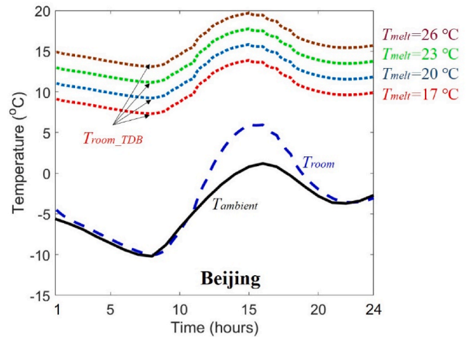
Fig. 11. Zone air temperature variations of the house in Beijing with T_{melt} ranging from 17\text{ }^{\circ}\text{C} to 26\text{ }^{\circ}\text{C} , and \epsilon = 0.4 .
