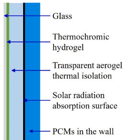
Fig. 2. A TDB integrated into the building envelope for energy savings.
