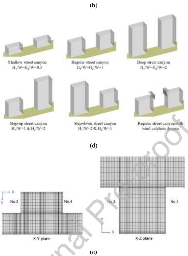
Fig. 2 (a) Model in the wind tunnel test, (b) CFD model description and boundary conditions, (c) setup of the target street canyon, (d) diagrams showing various target street canyon geometries, and (e) CFD grid arrangements of target street canyon for regular street canyon
