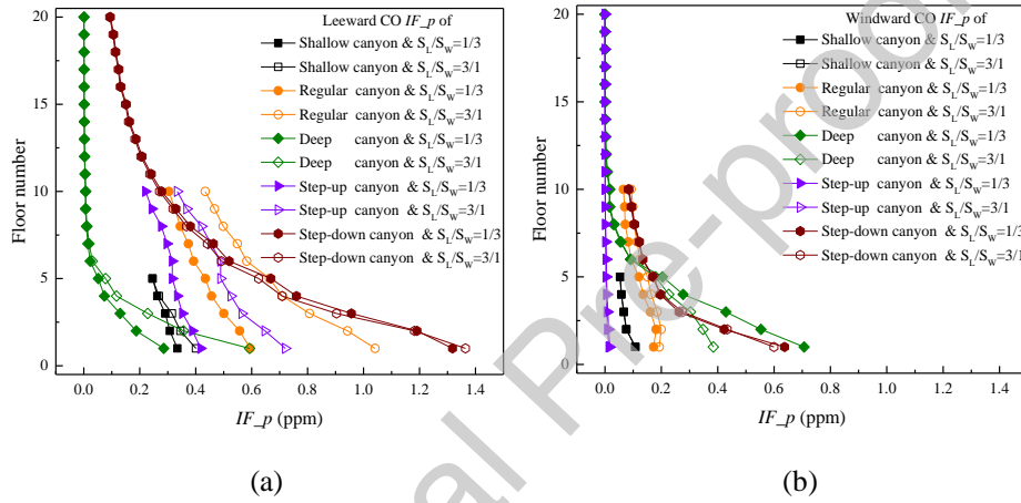
Fig. 6 Vertical profiles of CO IF_p in different floors in the street canyons with different geometries
