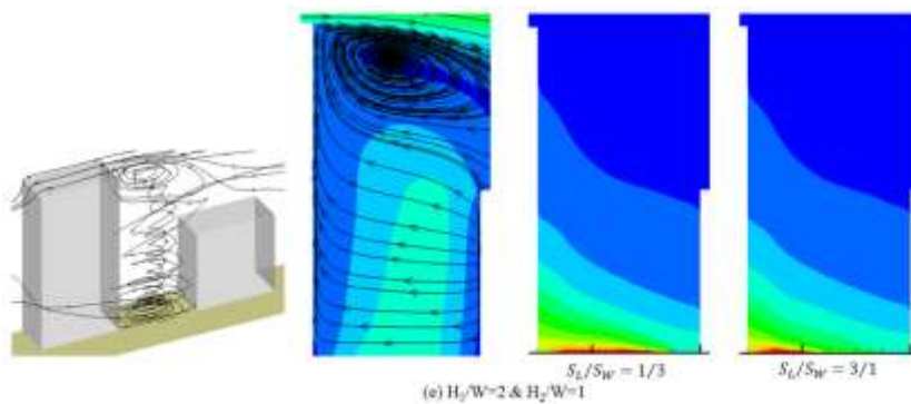
Fig. 4 3D streamlines, wind velocity, and CO concentration at y=30 m in
