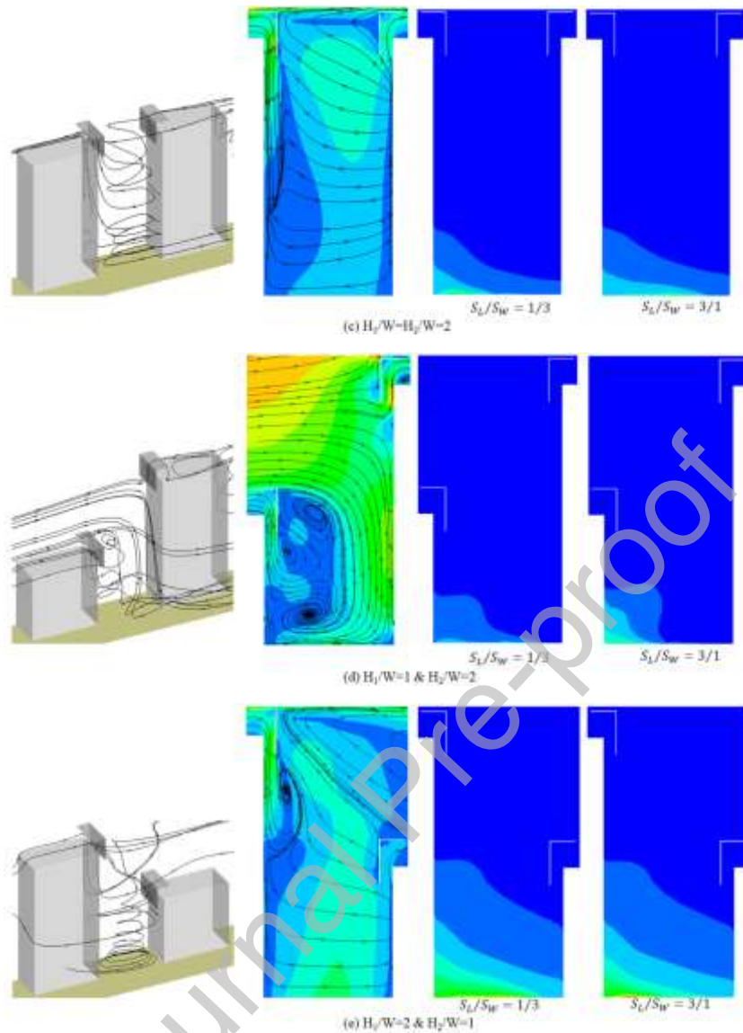
Fig. 7 3D streamlines, wind velocity, and CO concentration at y=30 m in the street canyons.
