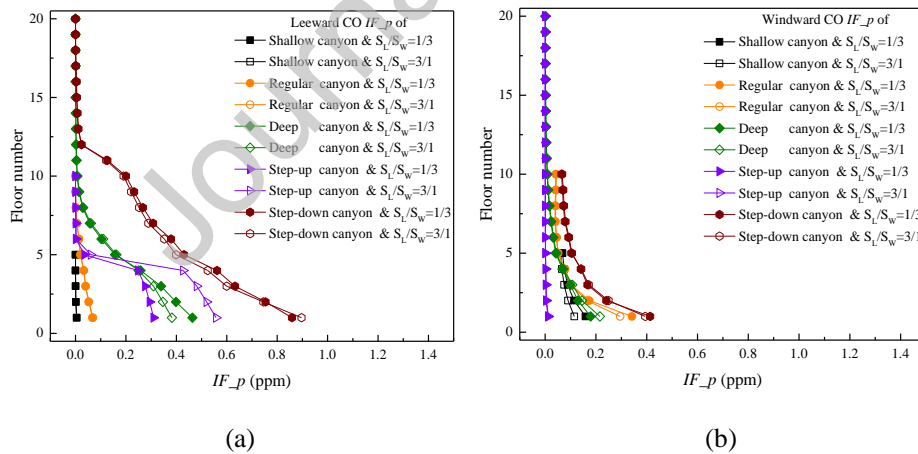
Fig. 8 Vertical profiles of the CO IF_p in different floors in the street canyons with different geometries with wind catcher design
